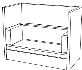
Art 05275: 1500x760 mm. Height 1198 mm.
