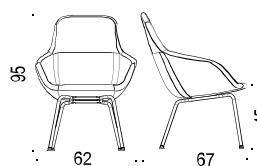
Art 20H/20M: 4-bent stålstativ, fast höjd / 4 metal legs, fixed height.
